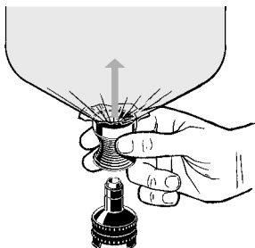
Detach Valve Balloon from Filling Chamber
