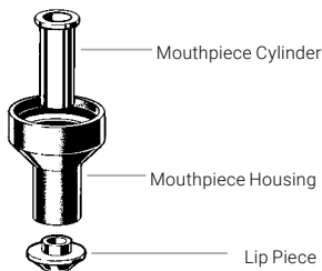
Pull off Lip Piece
